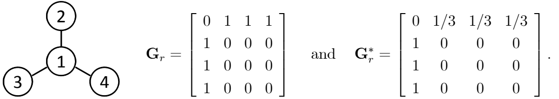
Figure 2: An example where the local-aggregate model can be identified but not the local-average model
