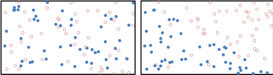
Figure 1: Randomness versus non-randomness
