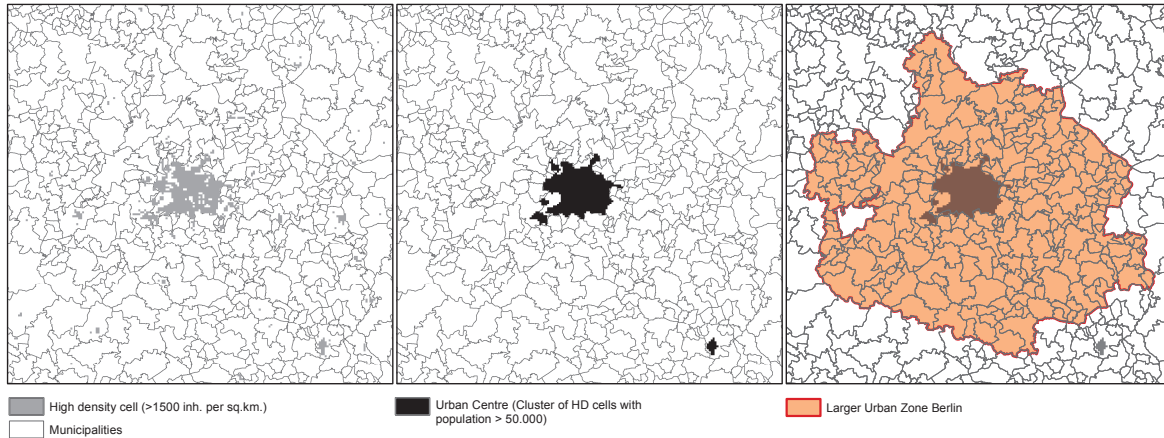
Figure 17.1: Construction of the Berlin functional urban area. Left panel shows the high-density cells with > 1500 inhabitants per square km and administrative municipal boundaries. Middle panel illustrates the construction of urban centers with total population > 50,000 . Right panel shows the construction of the larger urban zone based on bilateral commuting flows. Source: European Commission (DG Regional and Urban Policy).
